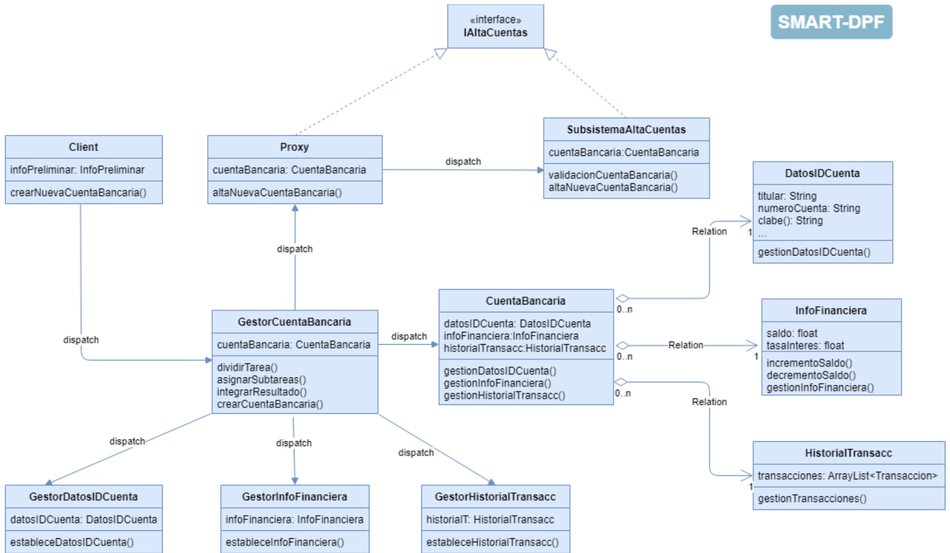
Figure 3: UML Diagram Bank System
