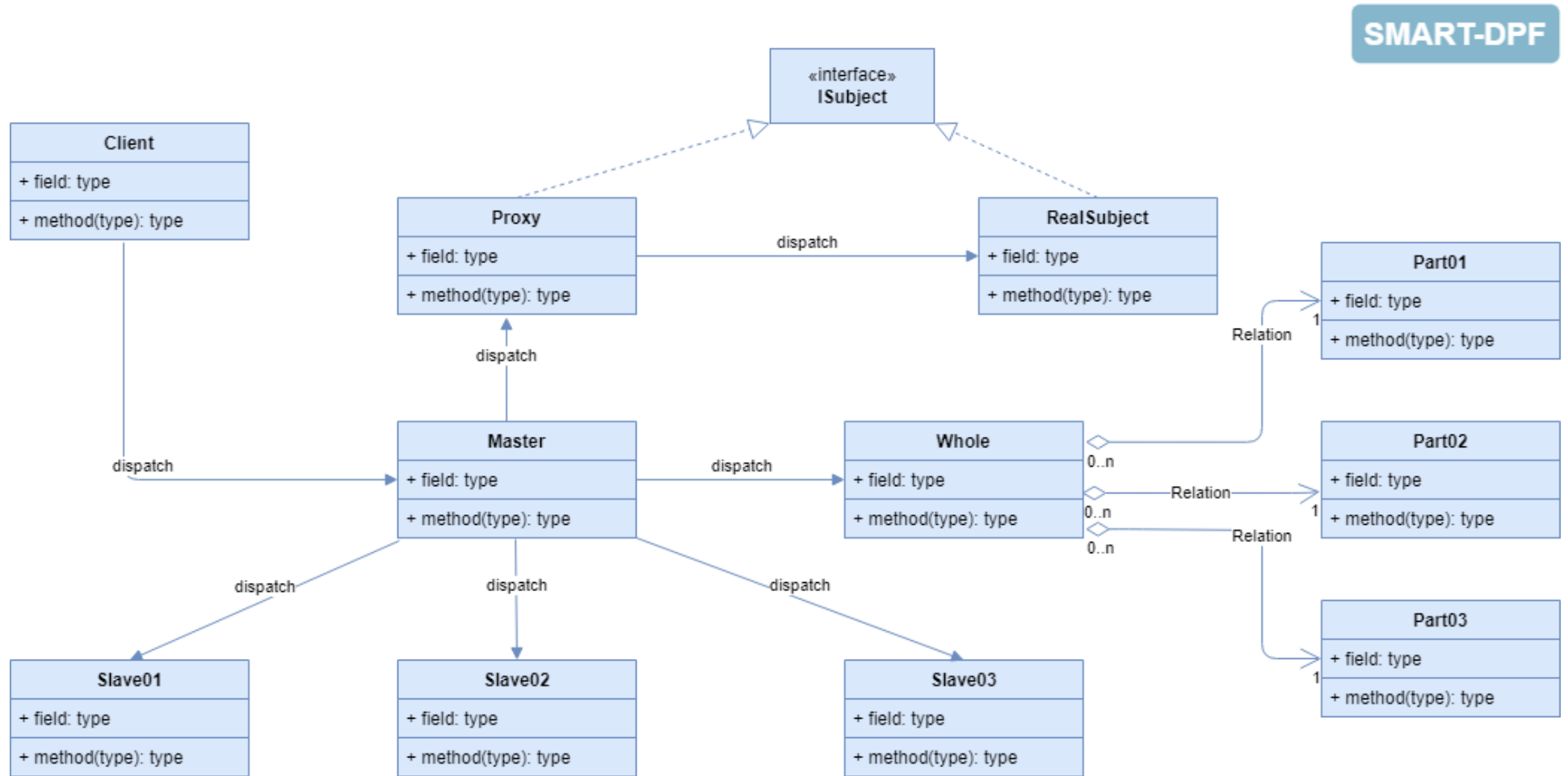
Figure 1: UML Diagram Whole-Part, Master-Slave and Proxy Pattern
