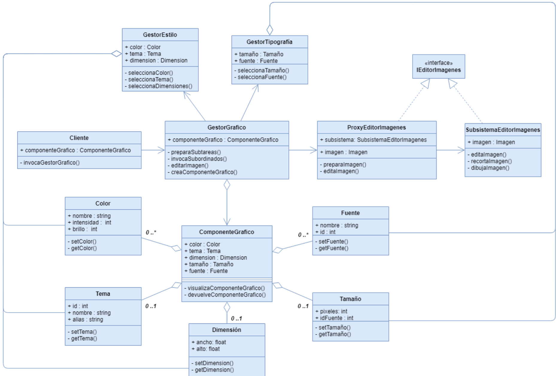
Figure 4: UML Diagram Dynamic Content Generator System
