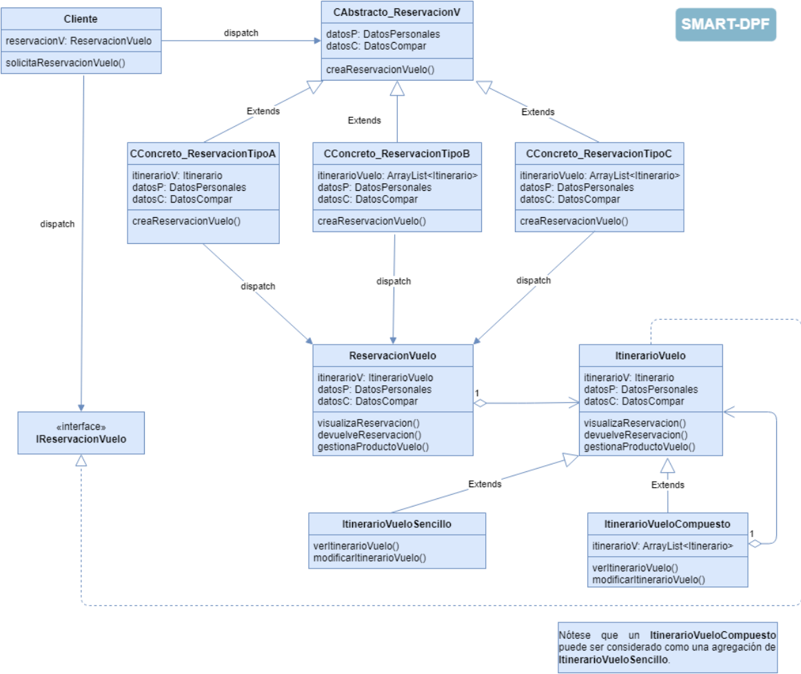
Figure 2: UML Diagram Travel Reservation System
