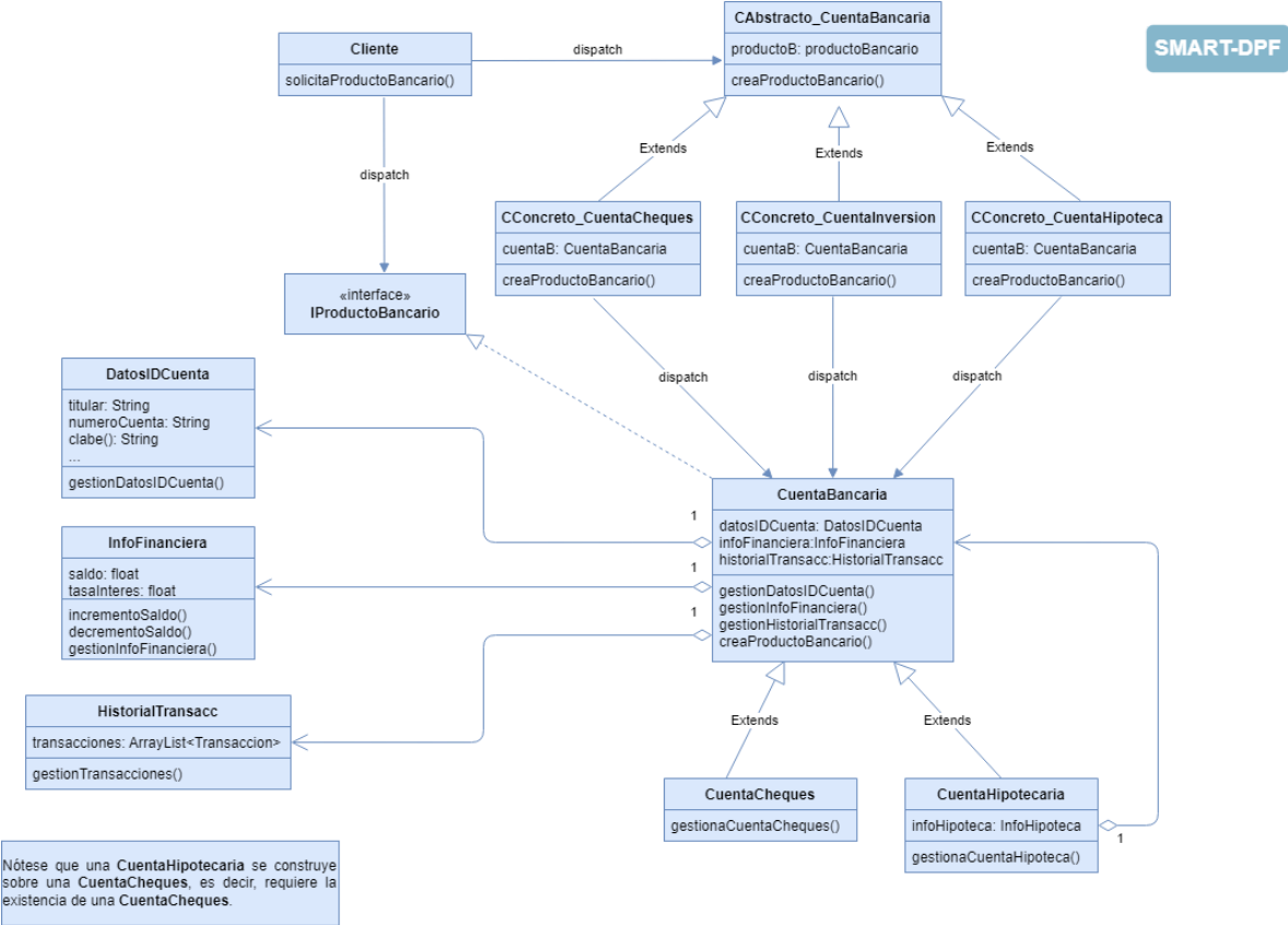
Figure 3: UML Diagram Bank System
