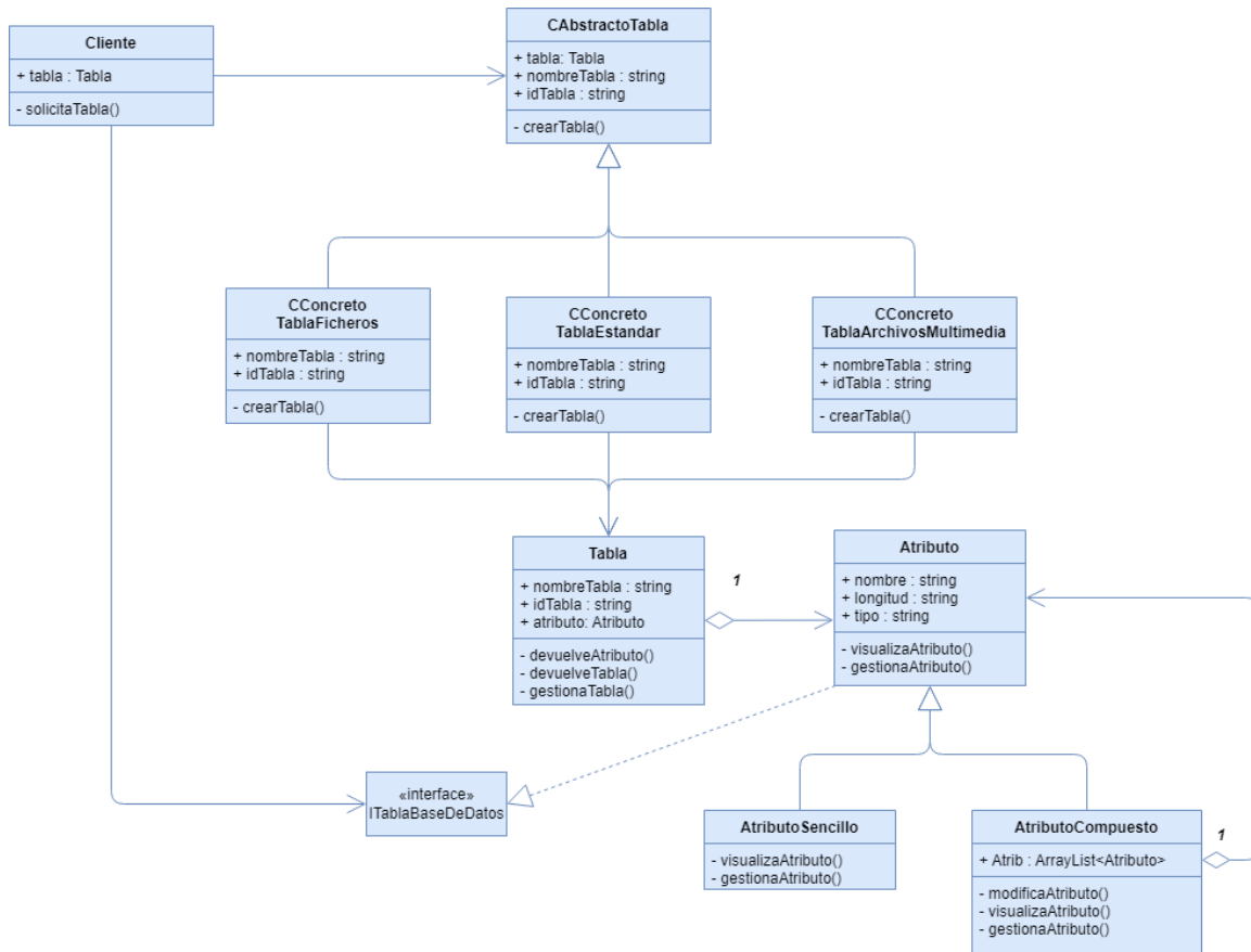
Figure 4: UML Diagram Dynamic Content Generator System
