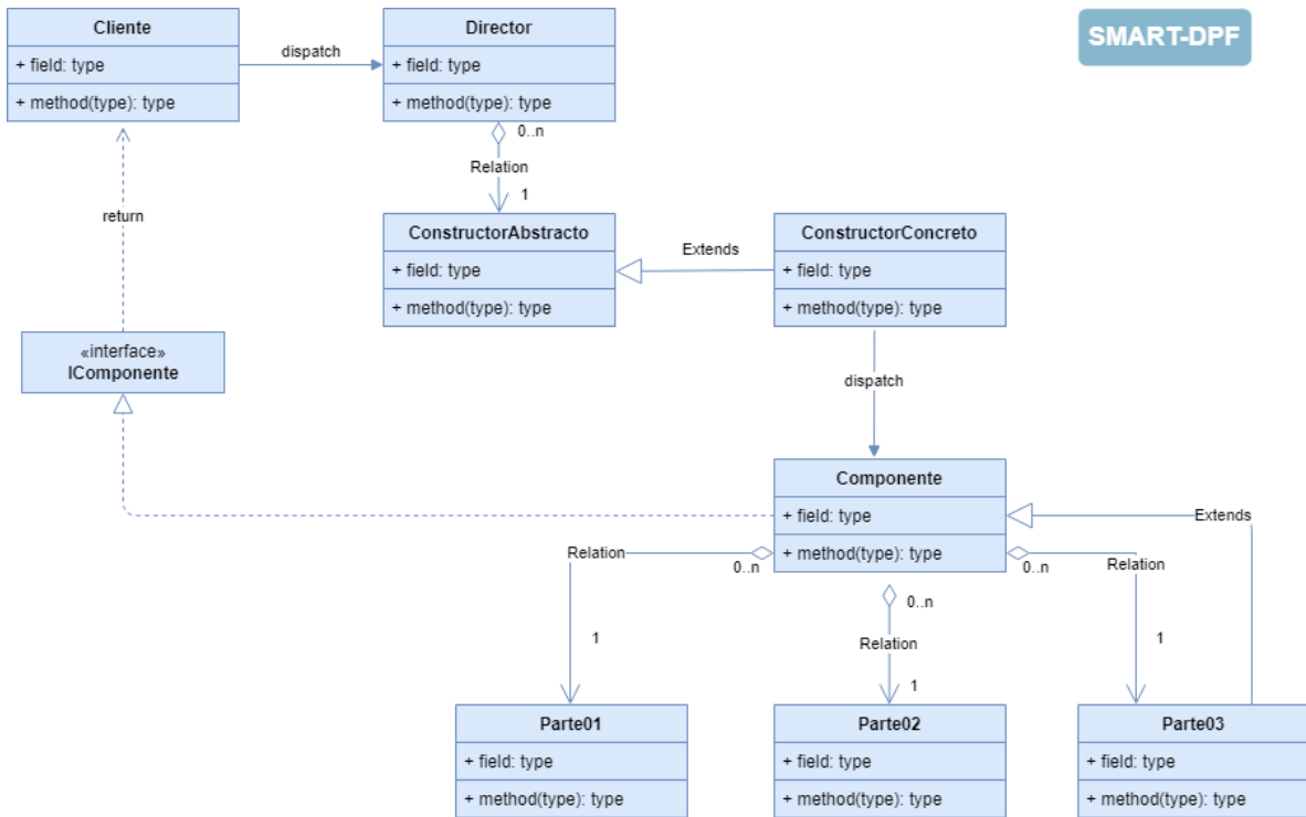
Figure 1: UML Diagram Builder and Composite Pattern
