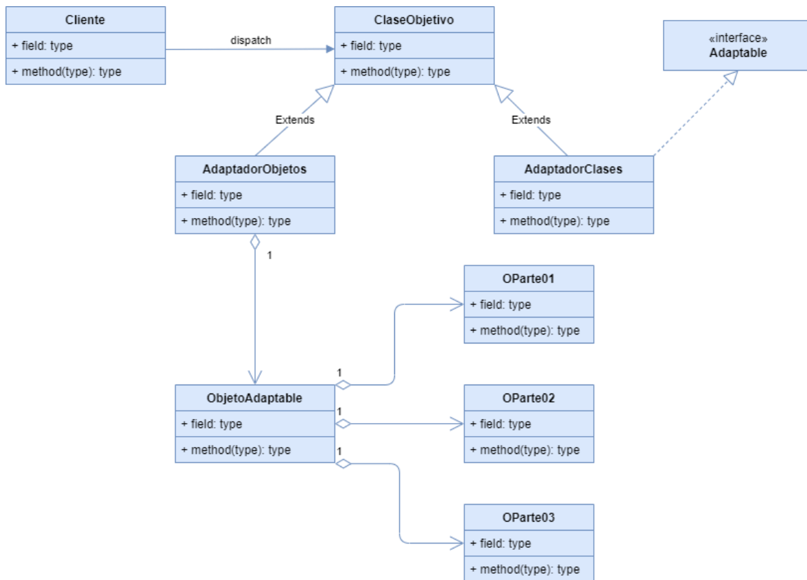
Figure 1: UML Diagram Adapter Object, Adapter Class and Whole-Part Pattern
