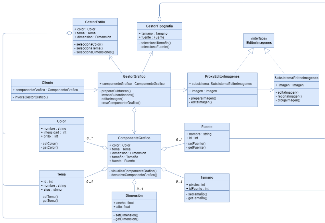
Figure 4: UML Diagram Dynamic Content Generator System
