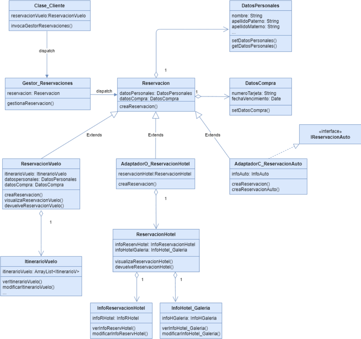
Figure 2: UML Diagram Travel Reservation System
