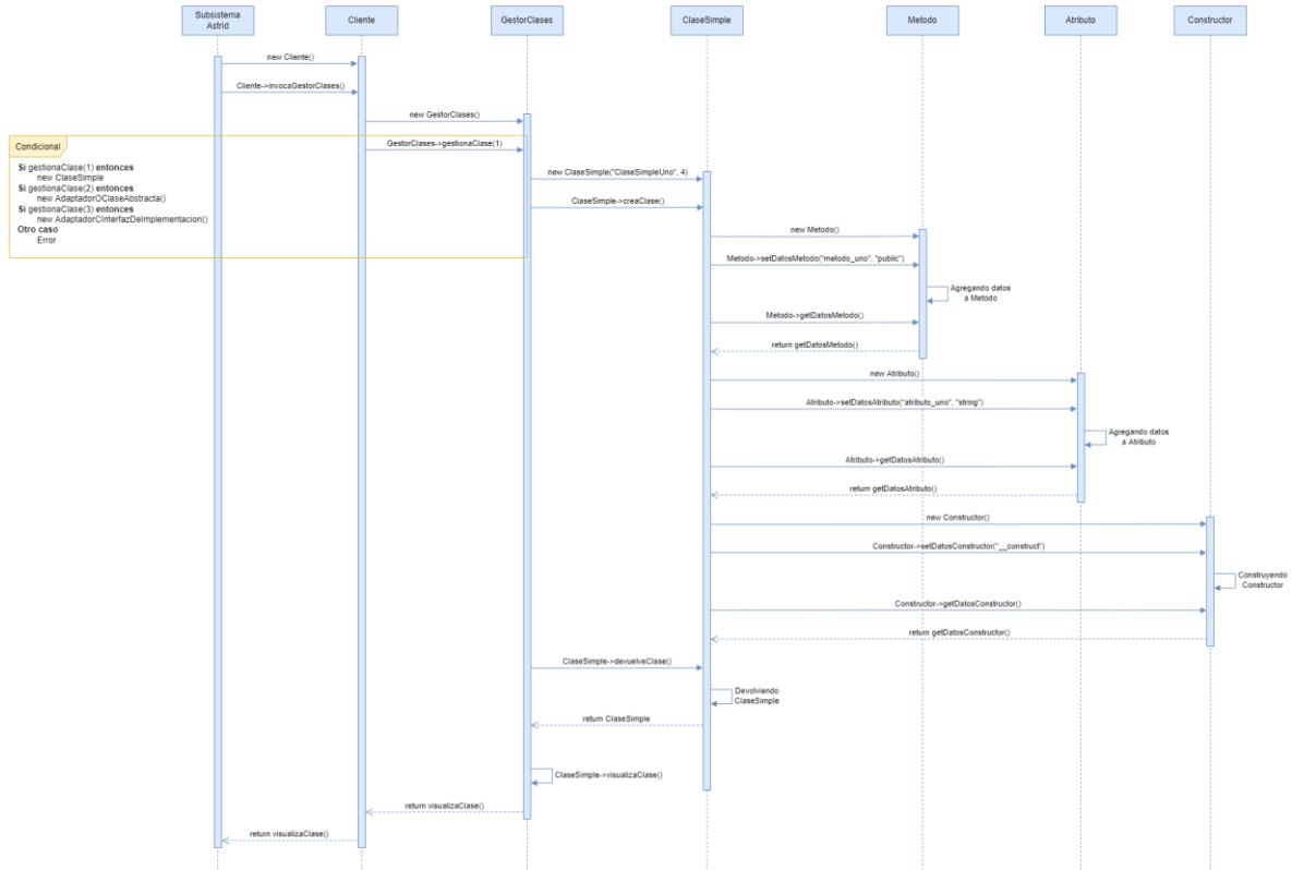
Figure 5: UML Diagram Dynamic Content Generator System
