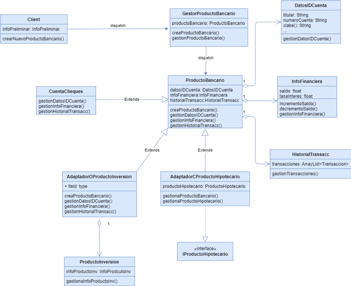
Figure 3: UML Diagram Bank System
