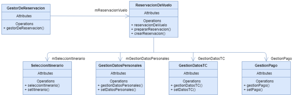
Figure 3: UML Diagram Flight System
