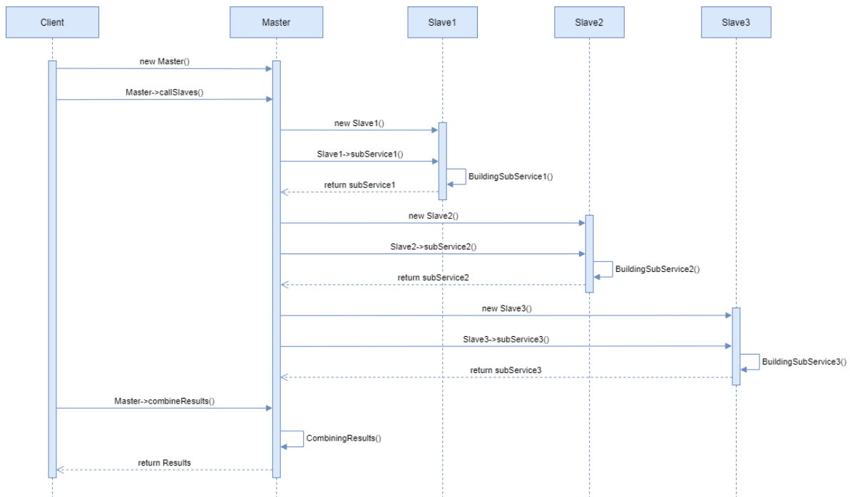
Figure 2: UML Diagram Master-Slave Pattern
