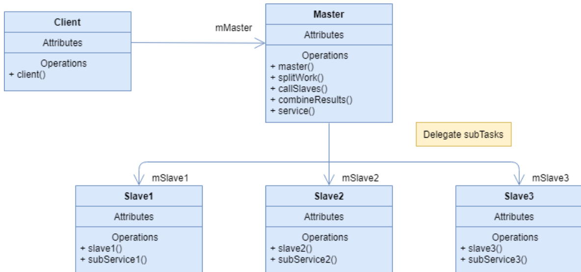
Figure 1: UML Diagram Master-Slave Pattern
