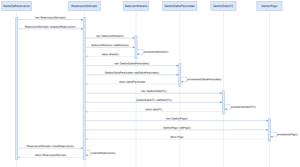
Figure 4: UML Diagram Flight System
